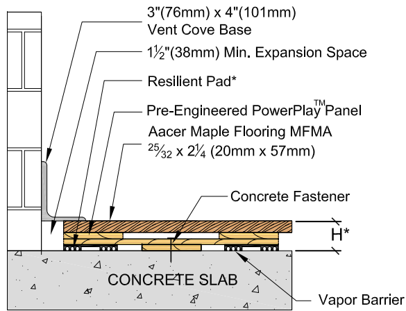
Wall Base
