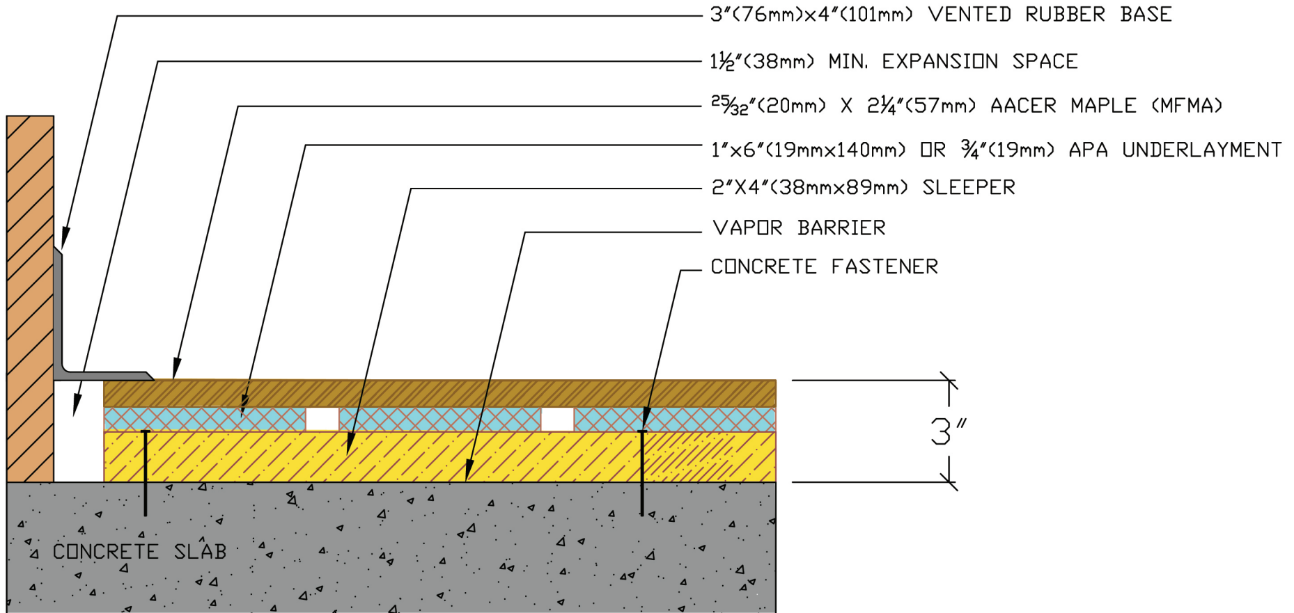
Wall Base Detail
