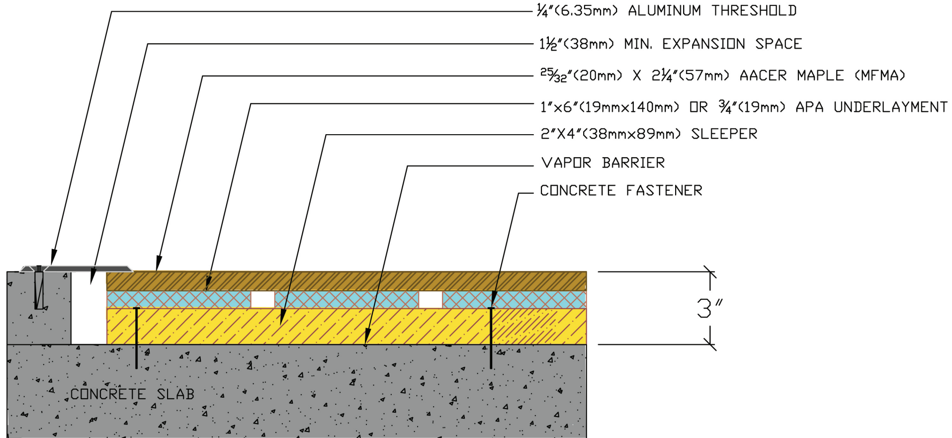
Threshold Detail
